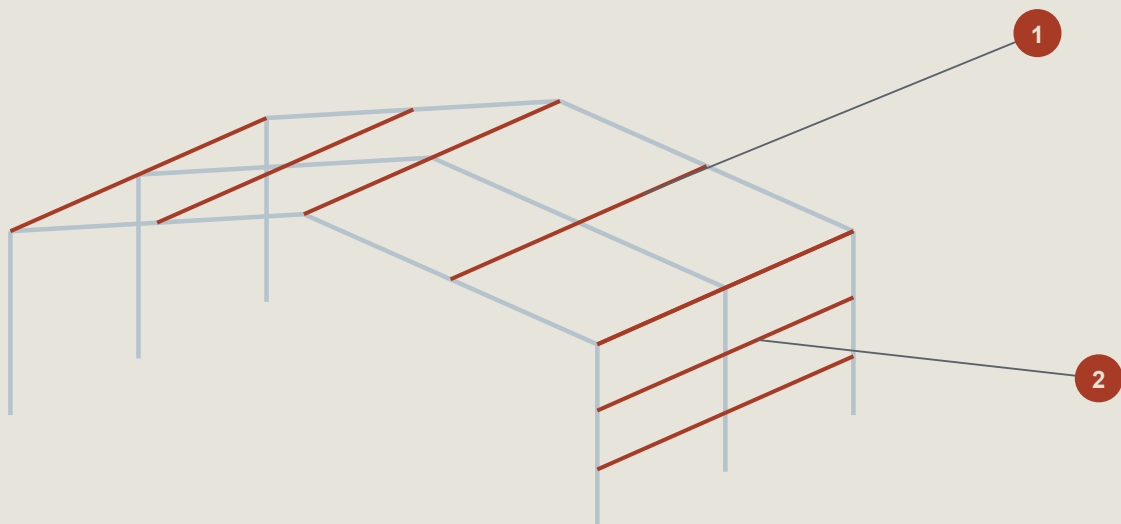
Roof framing detail / application reference
